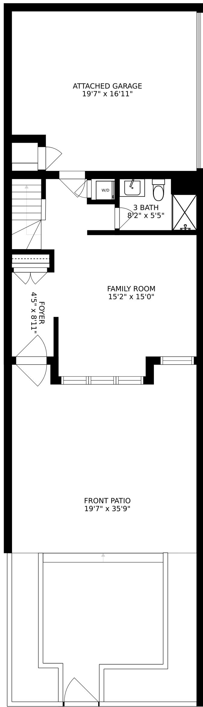
FLOOR 1
