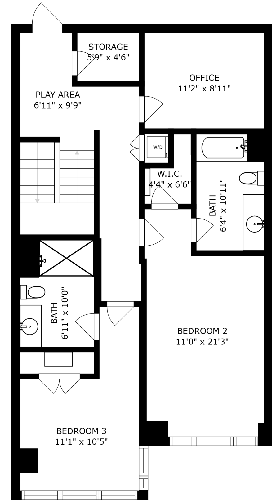
FLOOR 3
