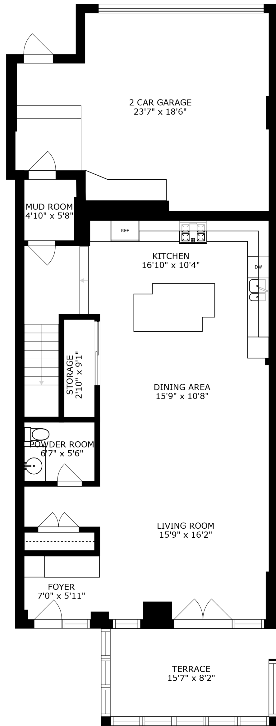
FLOOR 1
