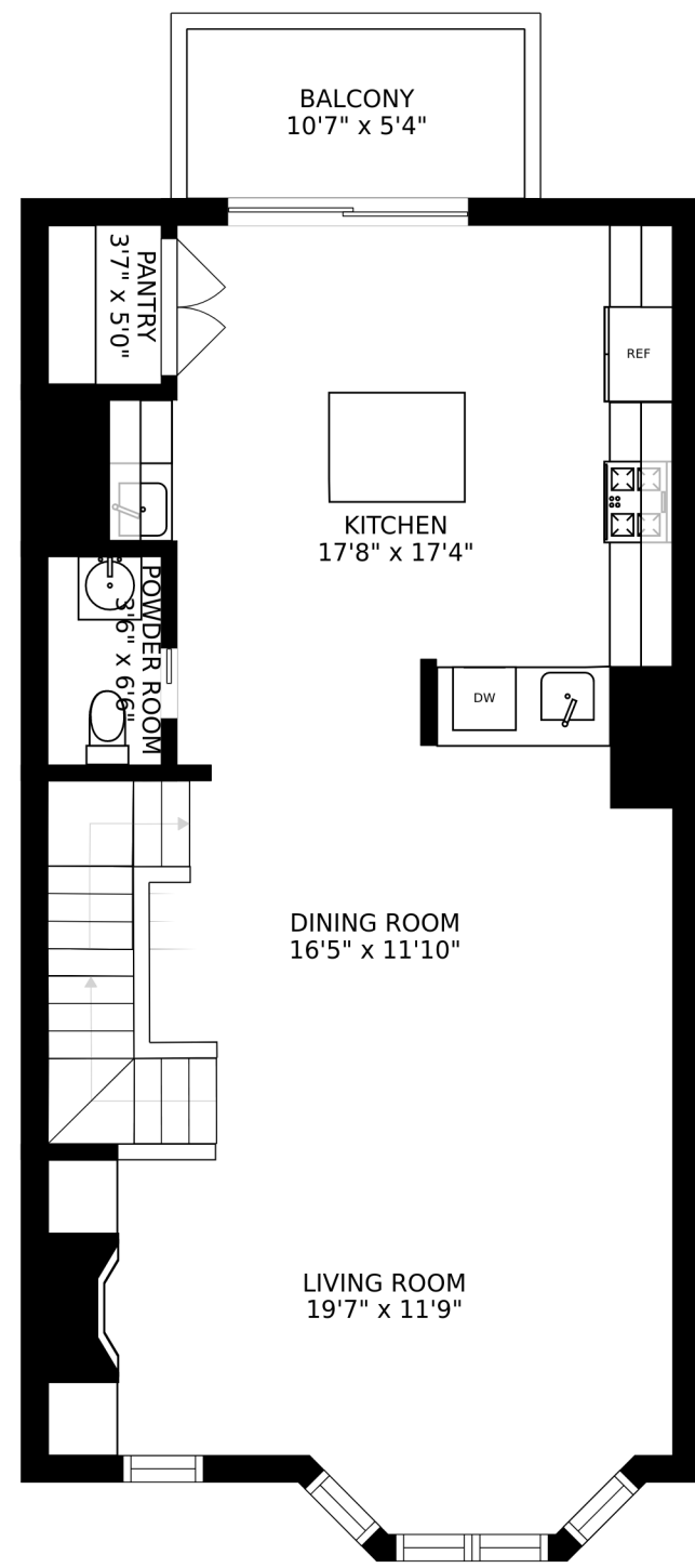
FLOOR 2
