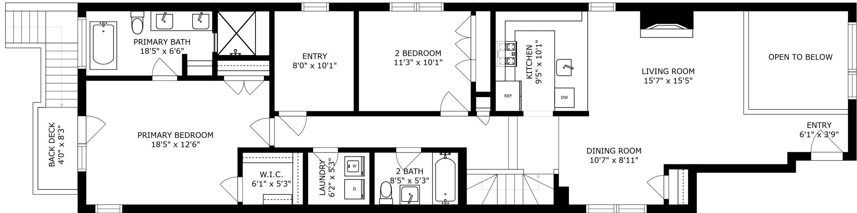
FLOOR 2
