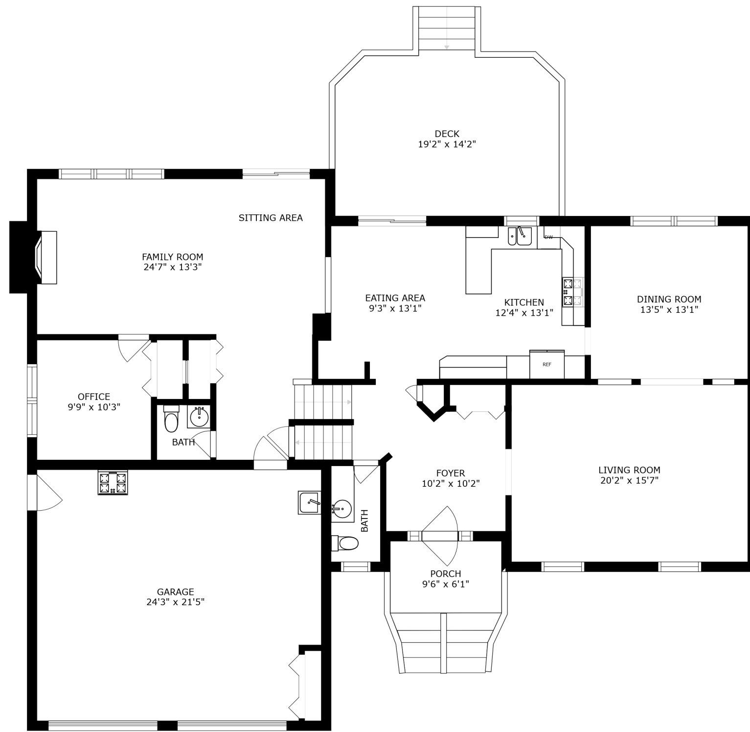
FLOOR 2
