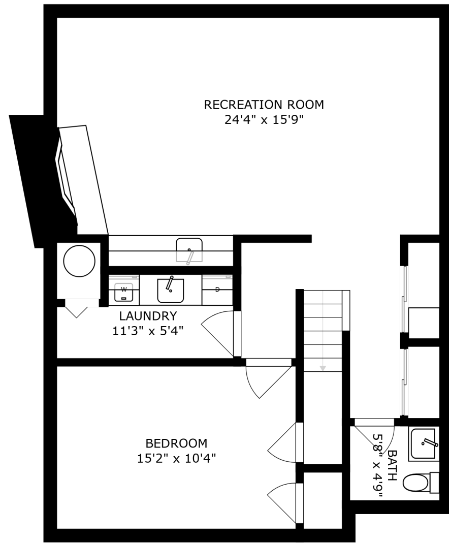
FLOOR 1
