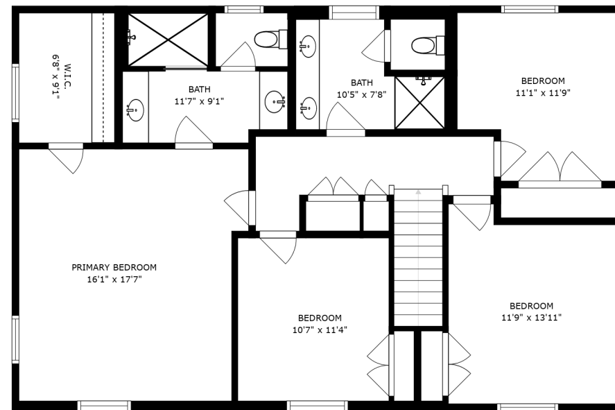
FLOOR 3
