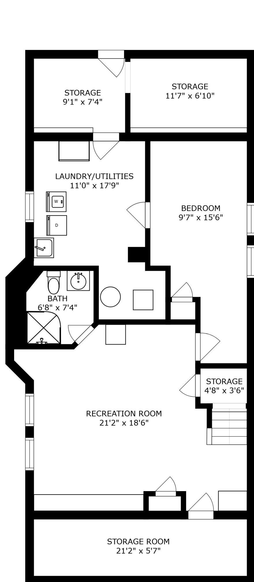
FLOOR 1
