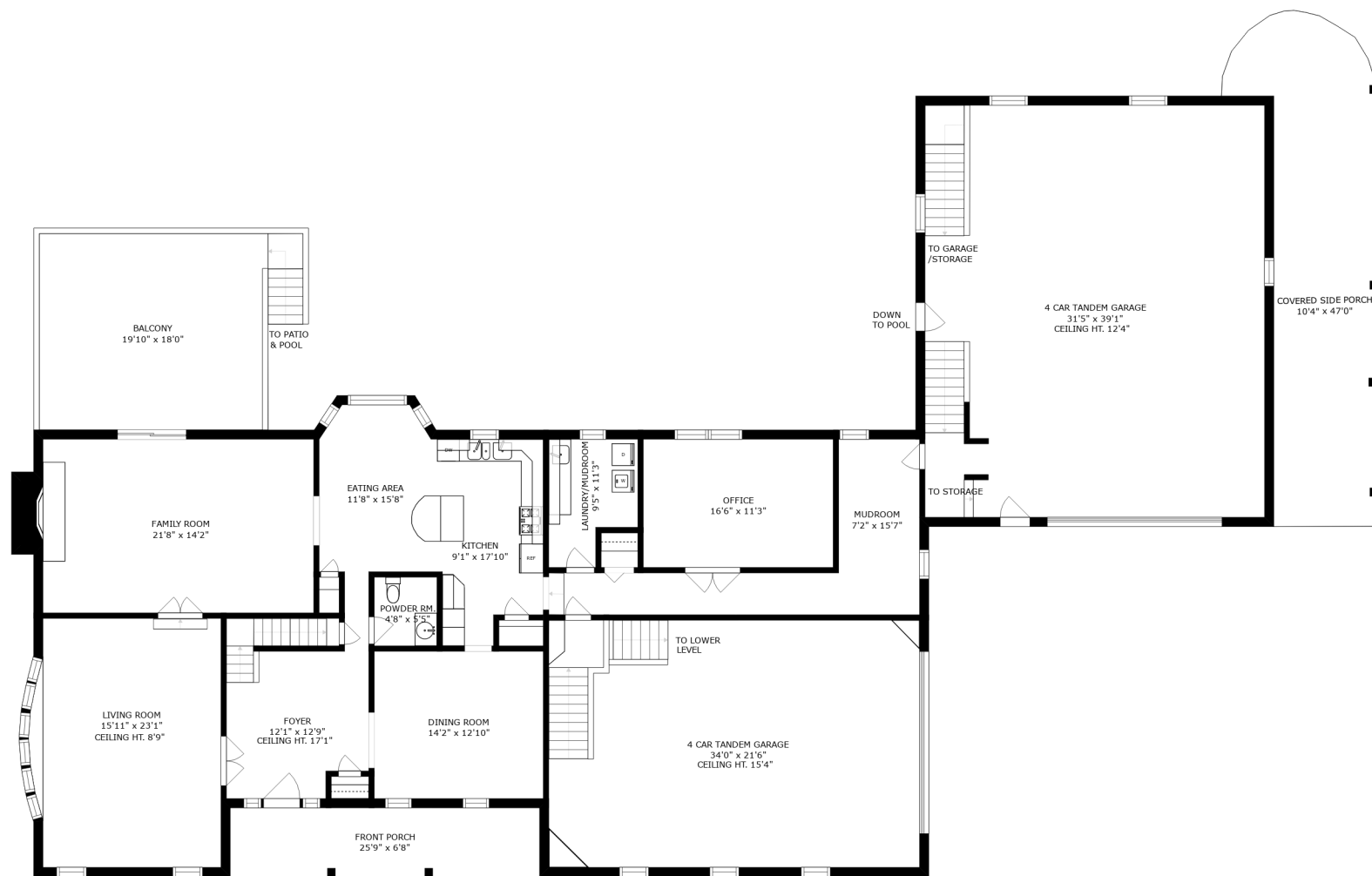
FLOOR 1 APPROX. INTERIOR SQ. FOOTAGE - 2,235 EXCLUDES 4 CAR TANDEM GARAGE - 748 & BACK 4 CAR TANDEM GARAGE - 1,248 CEILING HT. 8'0" UNLESS SPECIFIED
