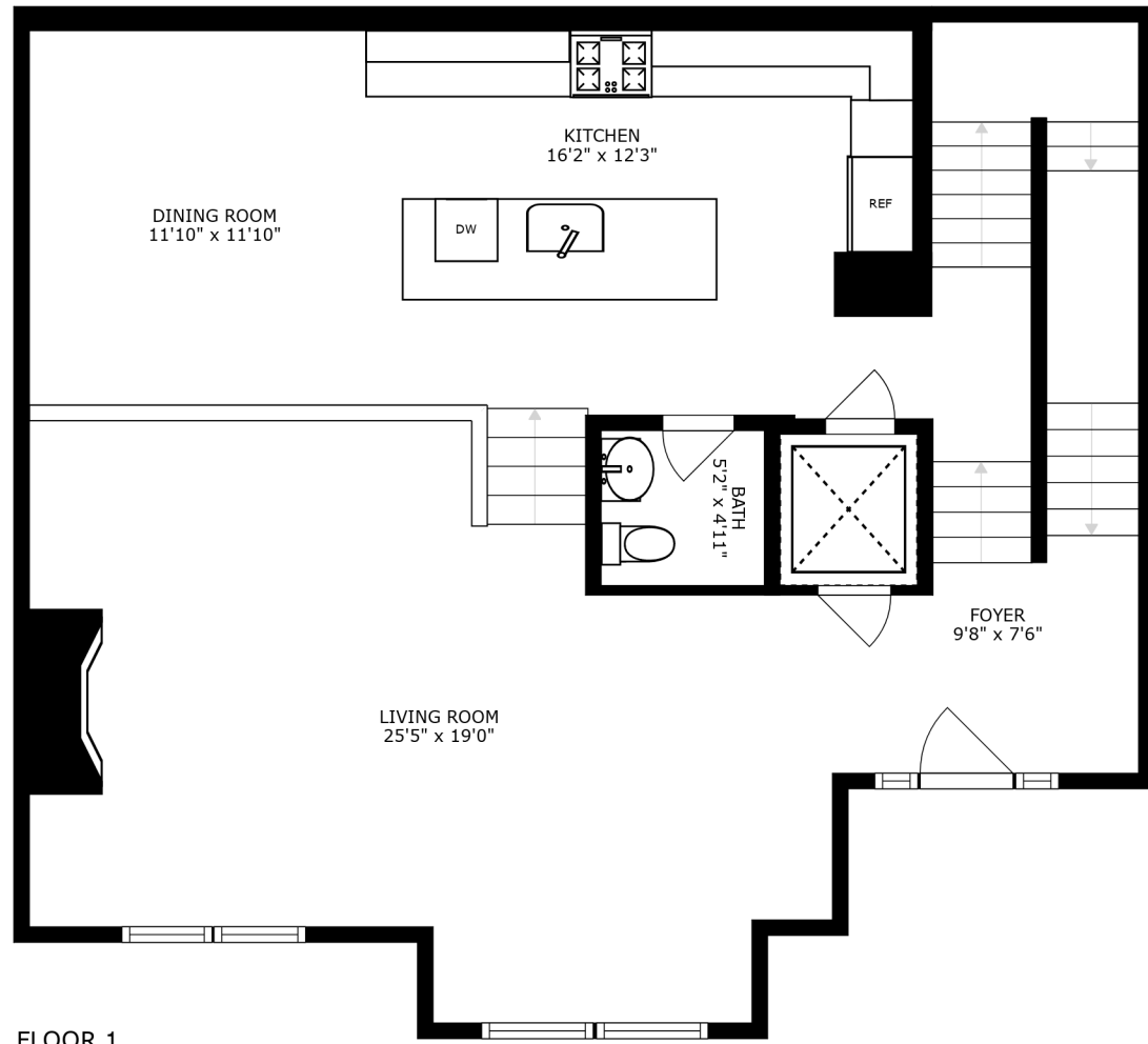
FLOOR 1
