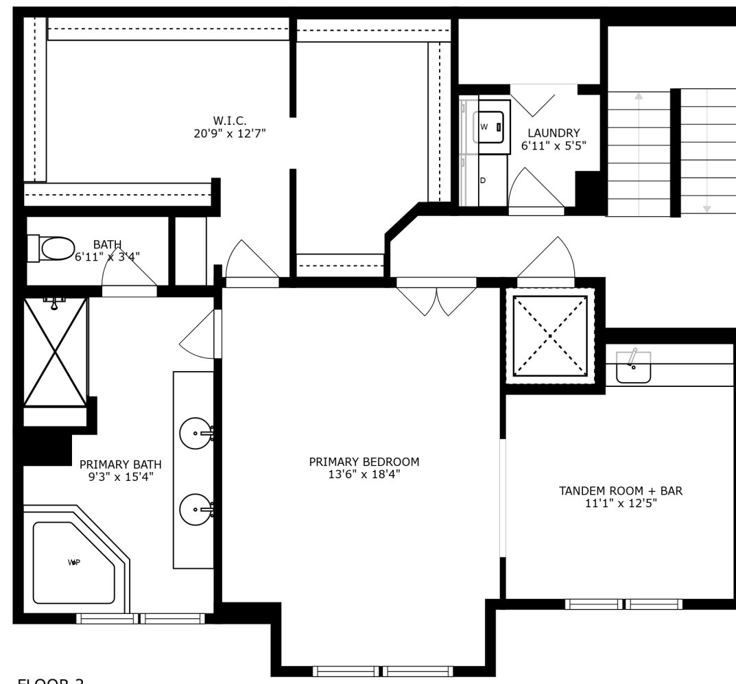
FLOOR 2
