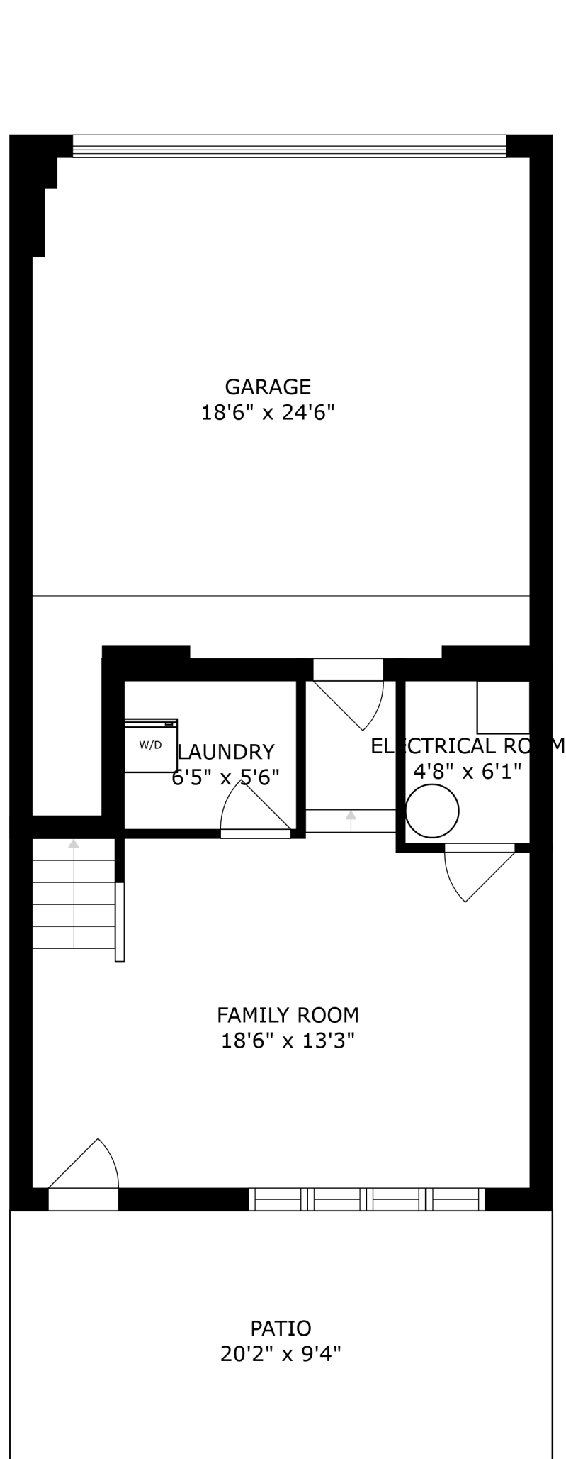
FLOOR 1
