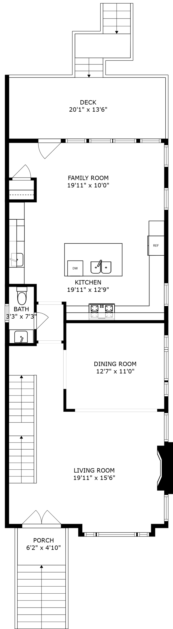
FLOOR 3
