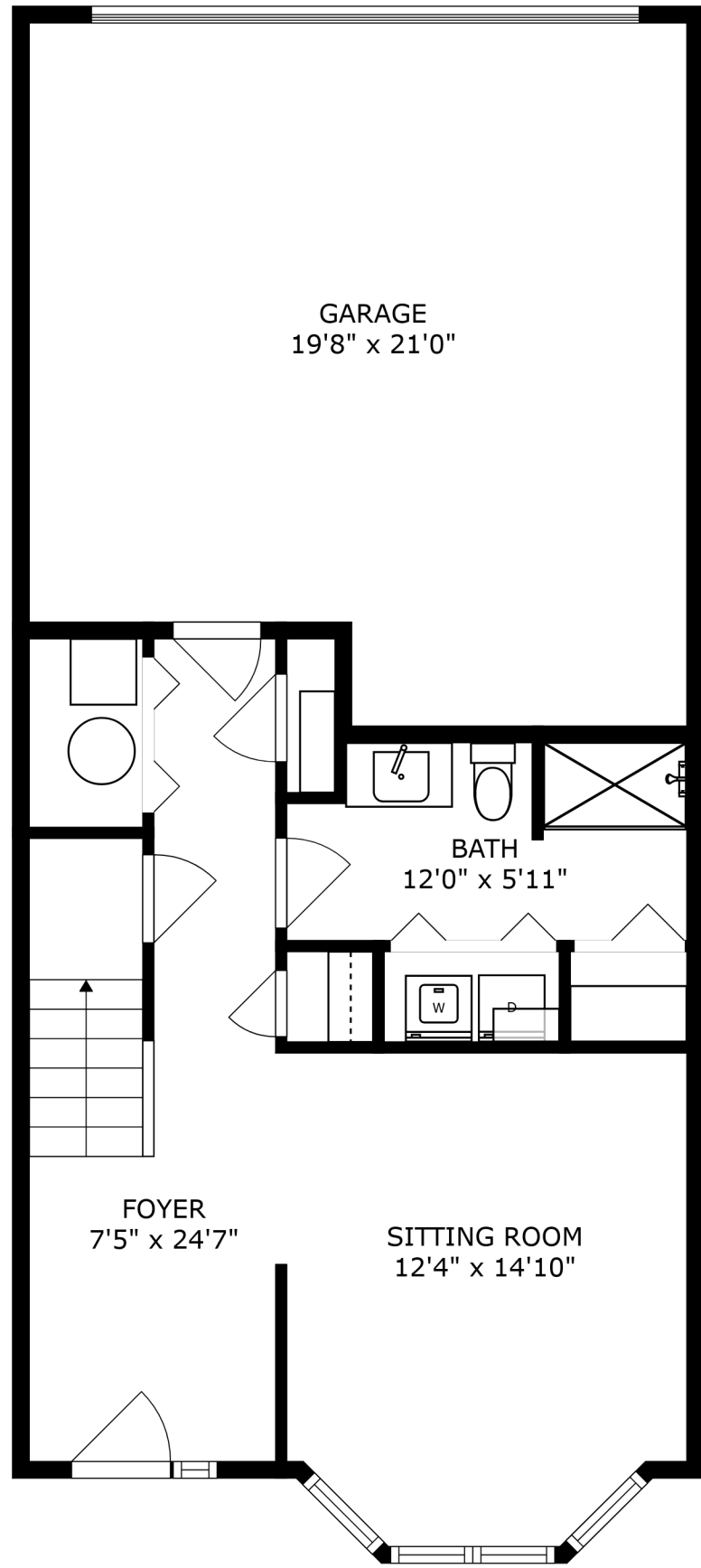
FLOOR 1
