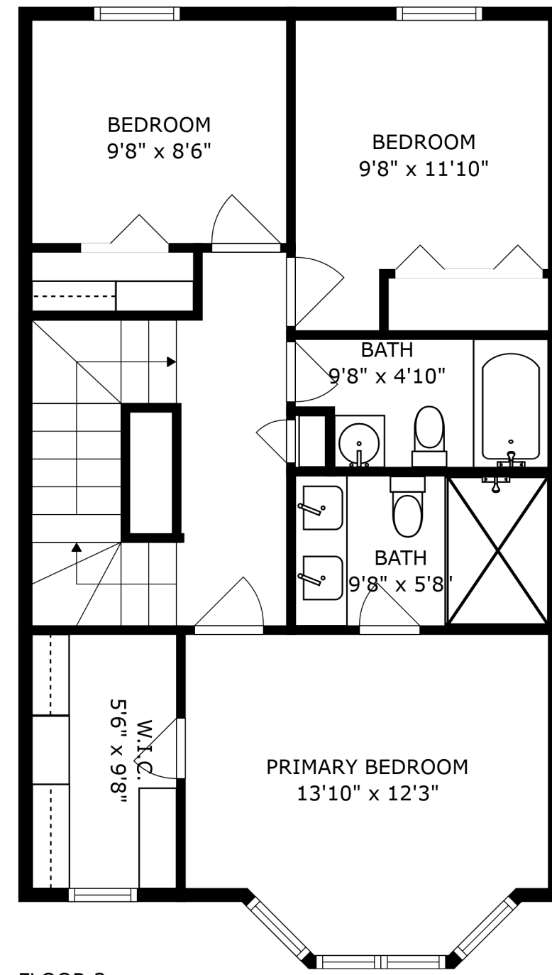
FLOOR 3
