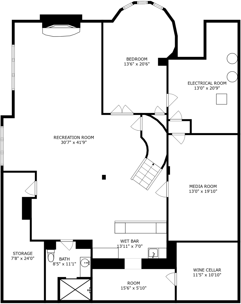
FLOOR 1
