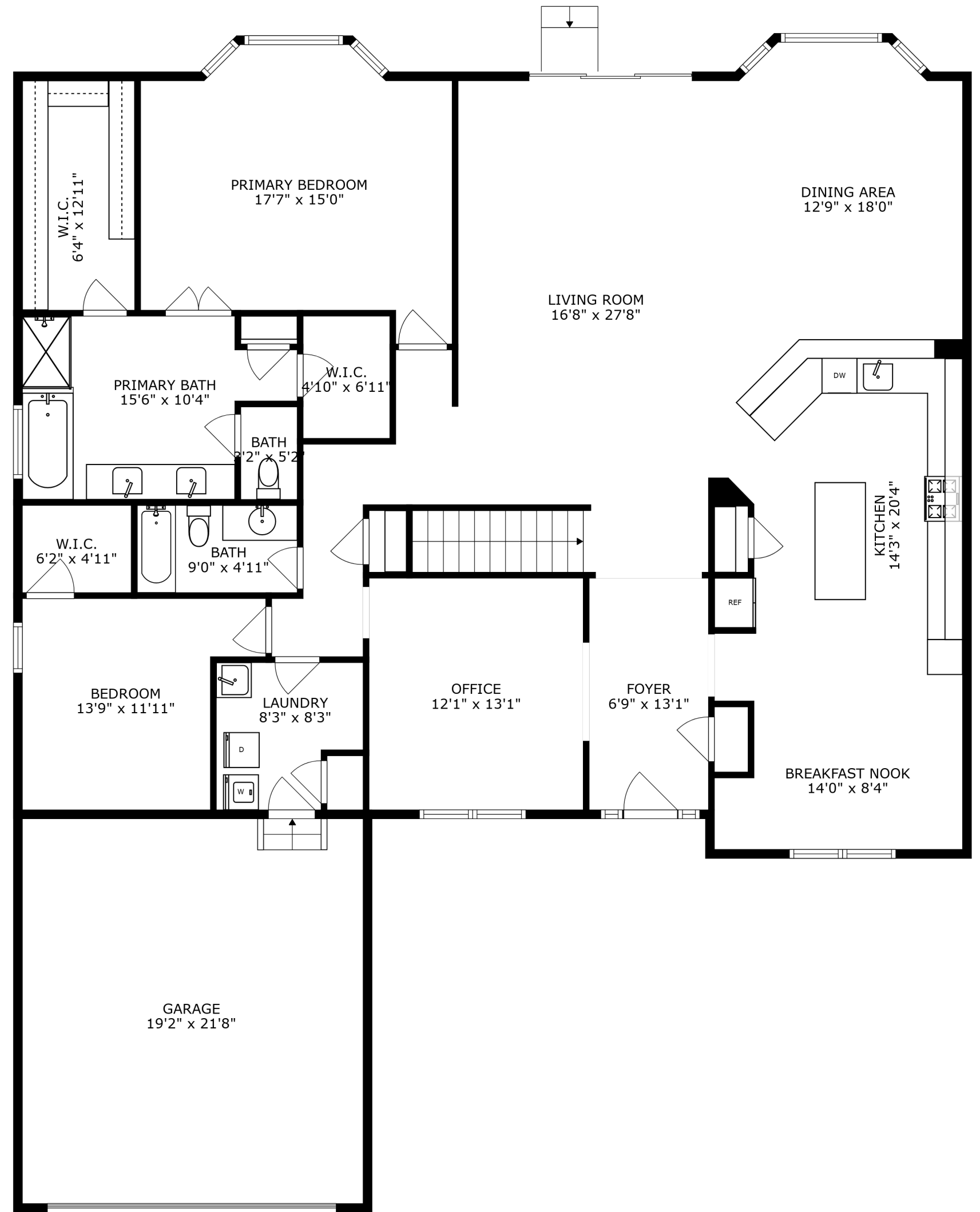
FLOOR 2
