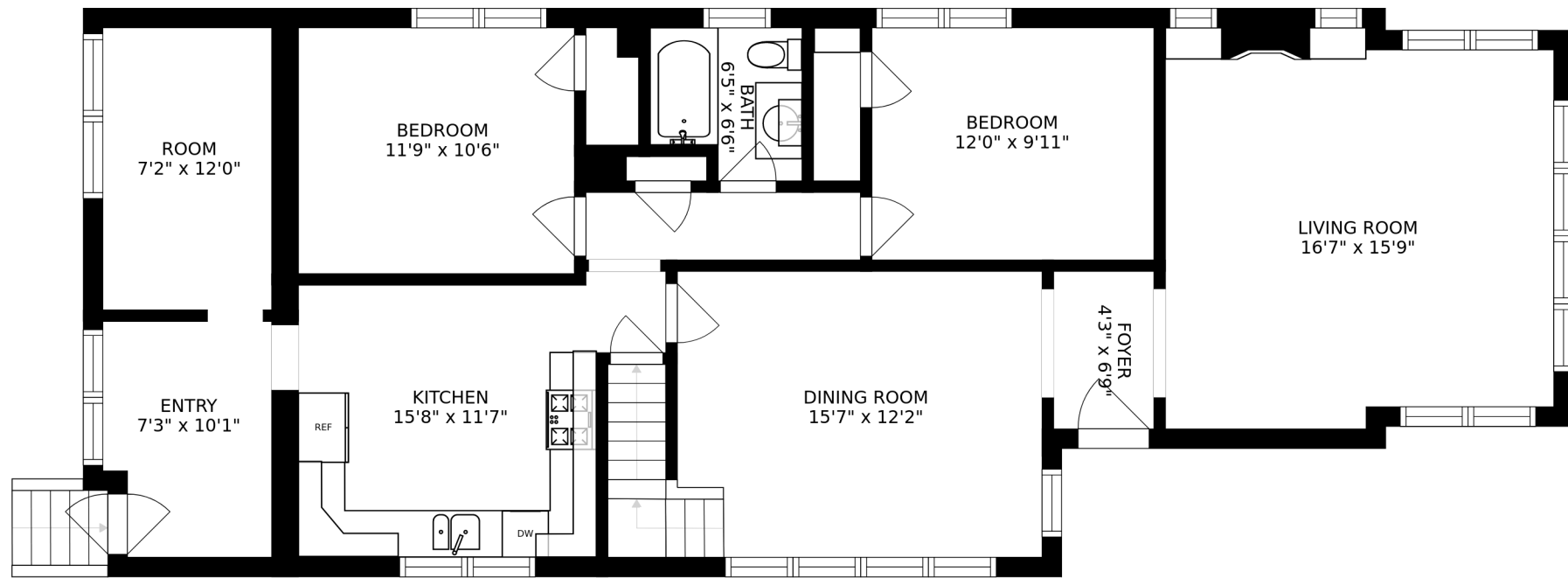
FLOOR 2
