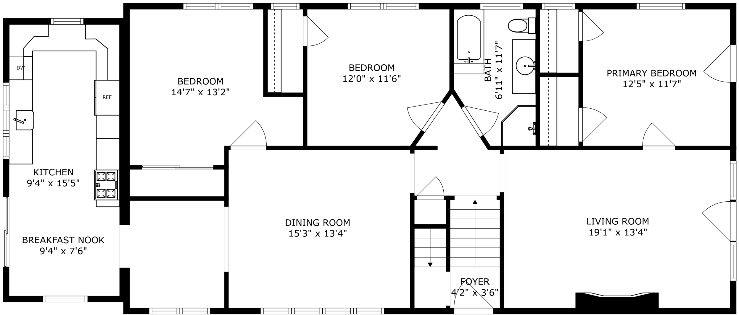
FLOOR 2
