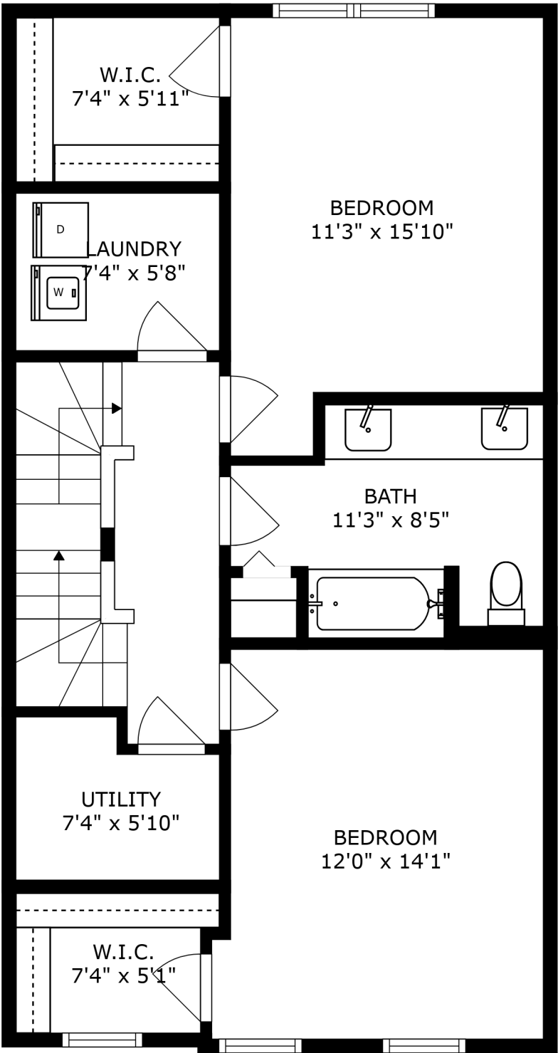
FLOOR 2
