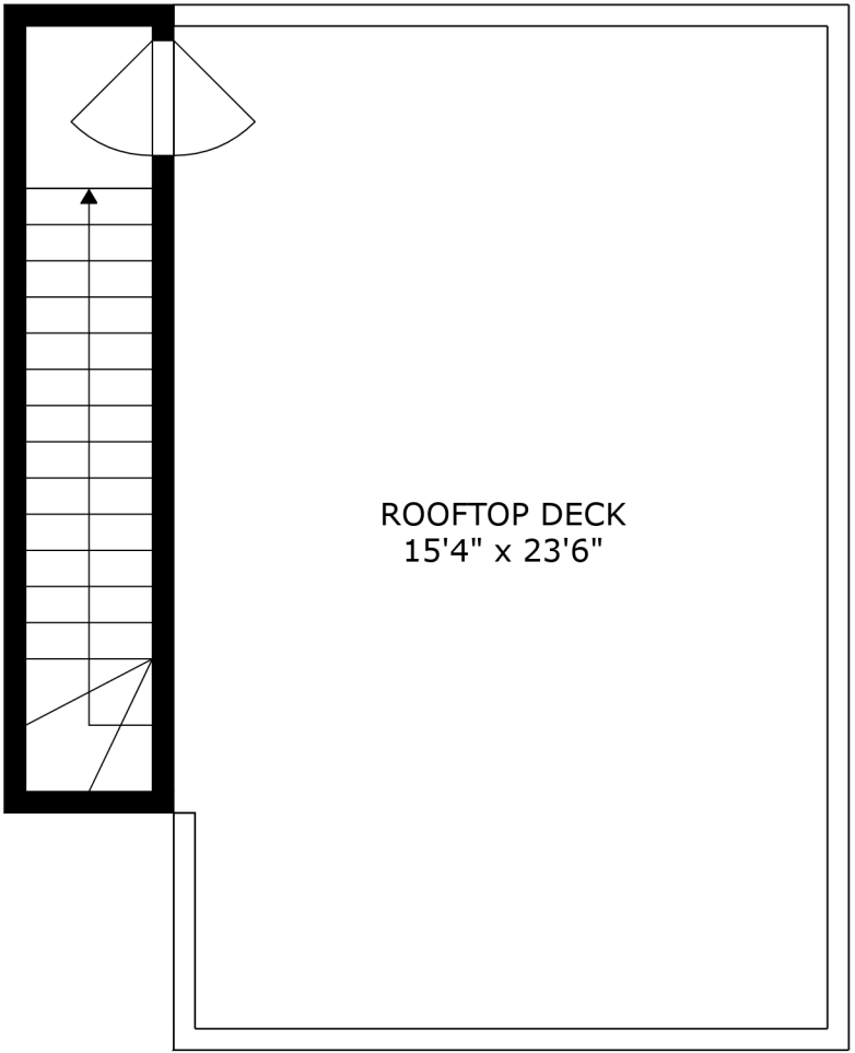
FLOOR 4
