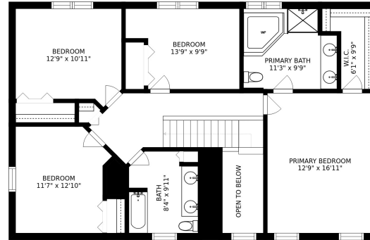
FLOOR 3
