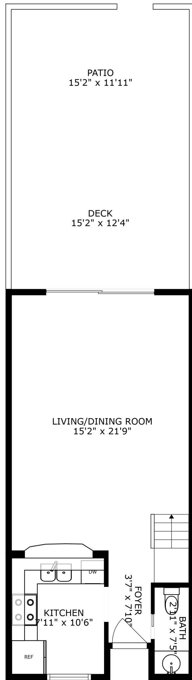
FLOOR 1
