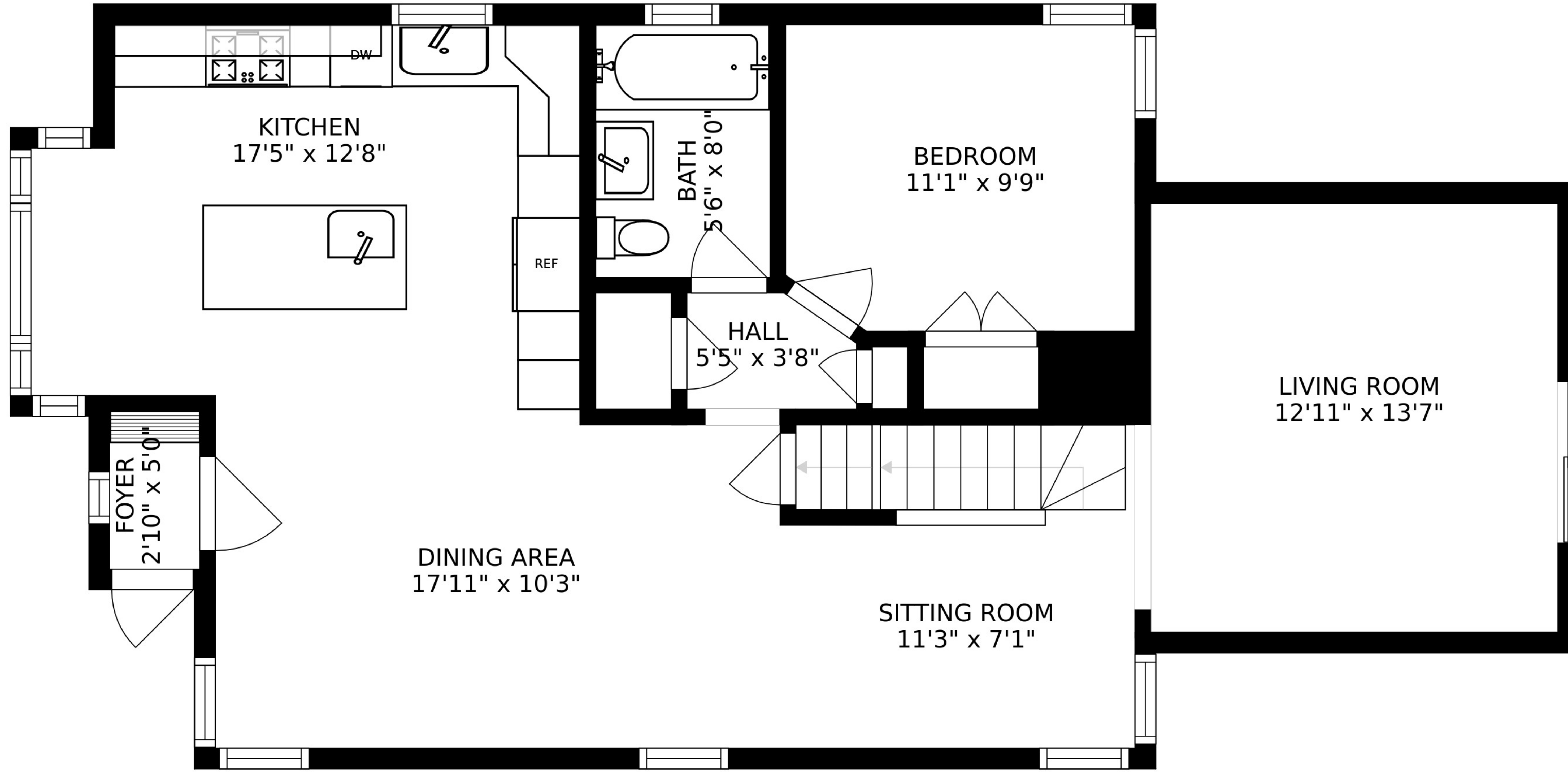
FLOOR 2
