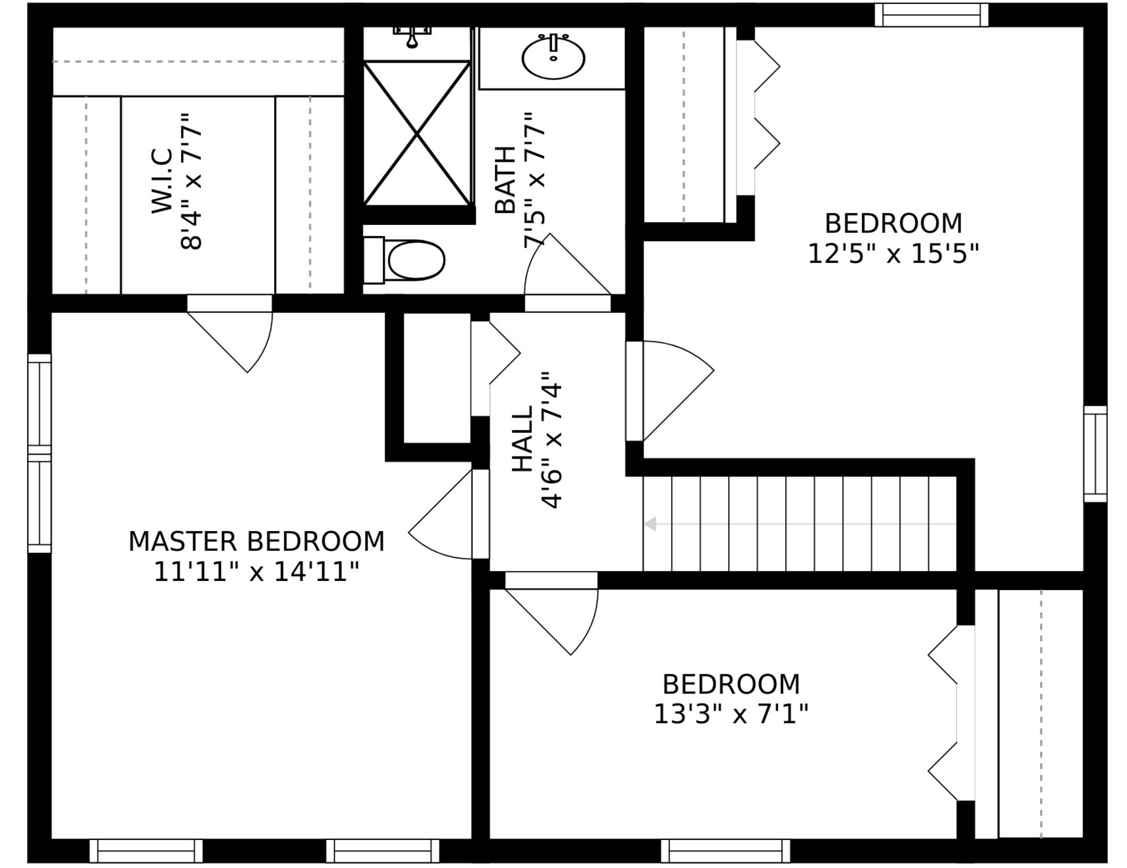
FLOOR 3
