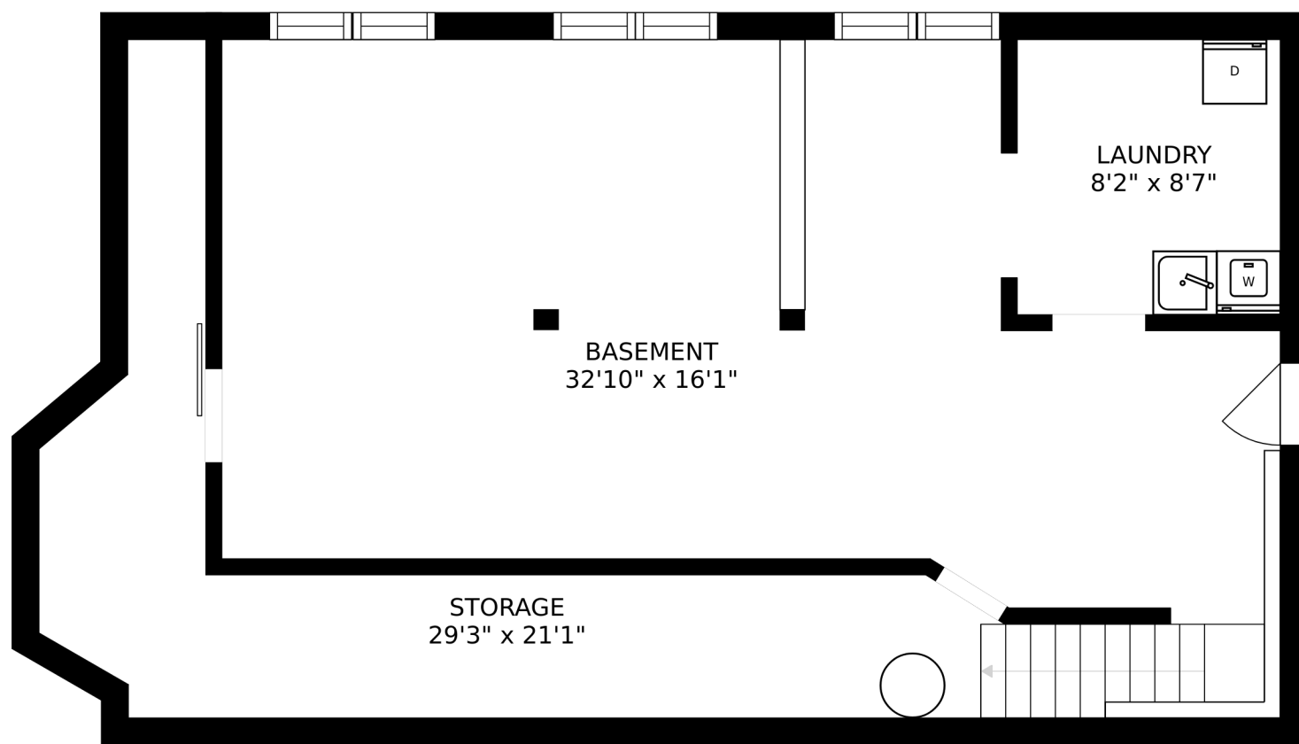
FLOOR 1
