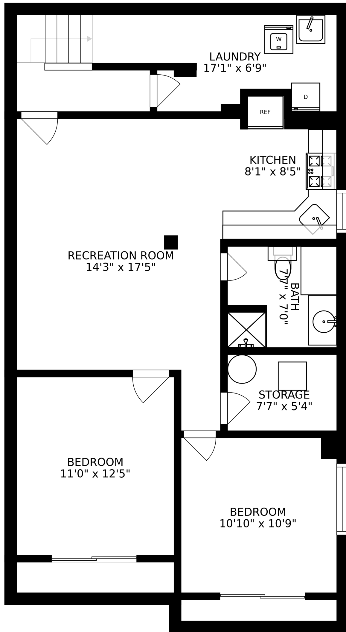
FLOOR 1
