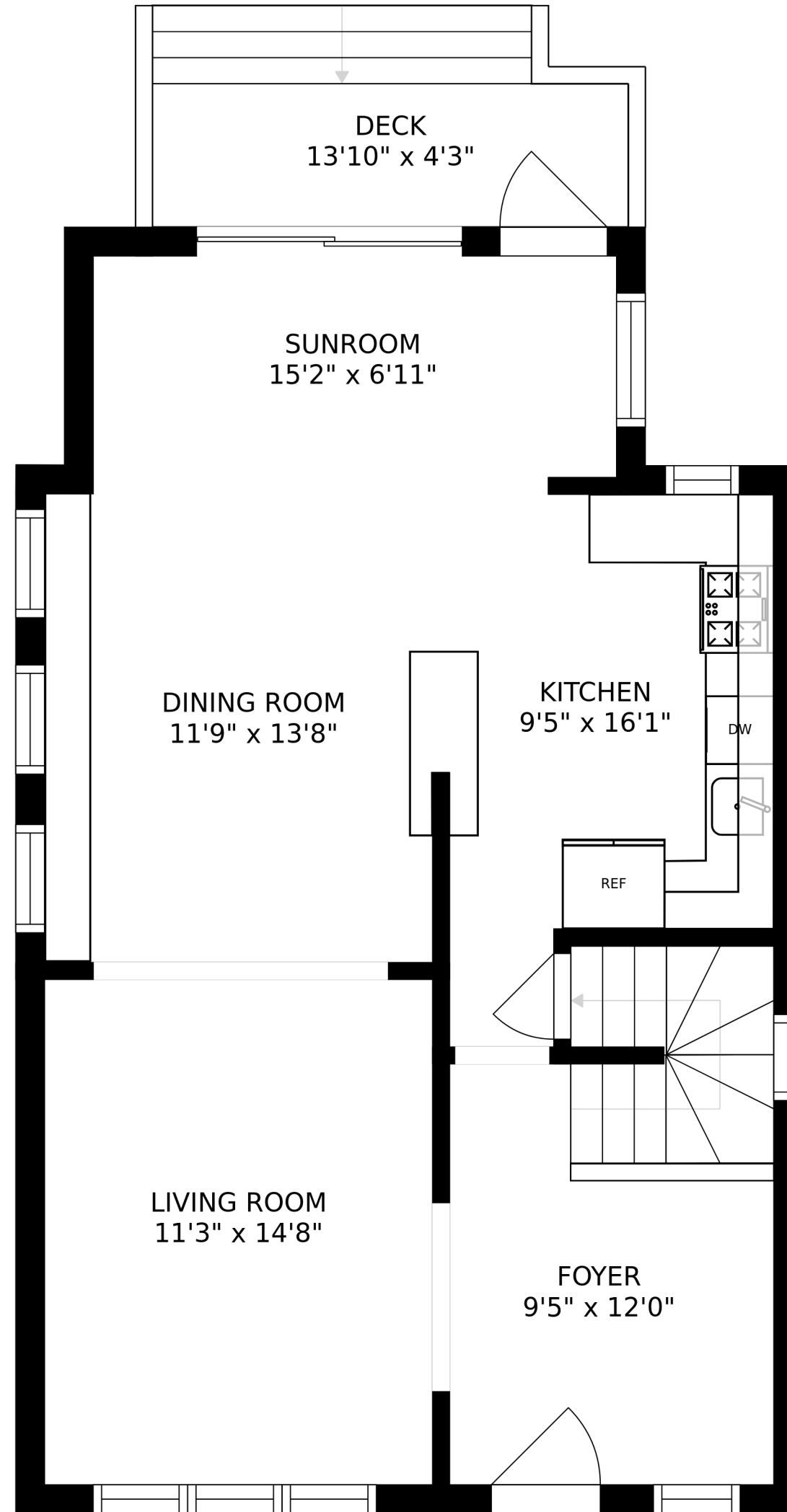
FLOOR 2
