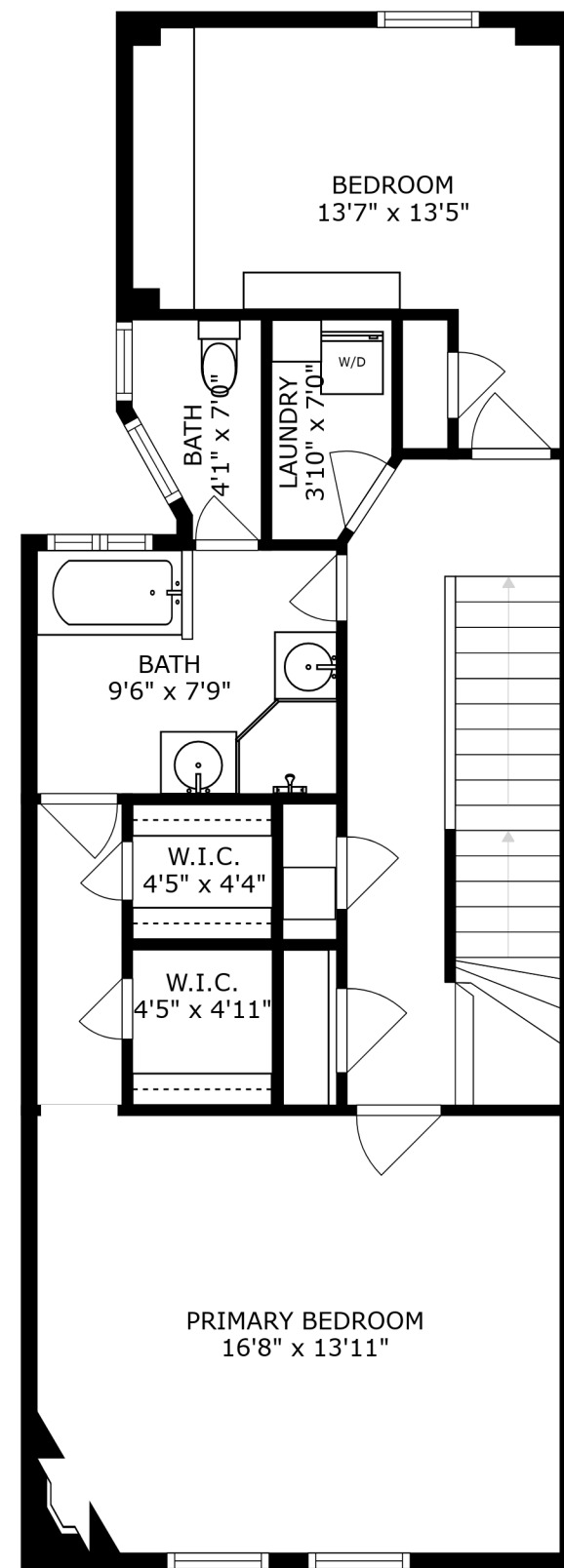
FLOOR 3
