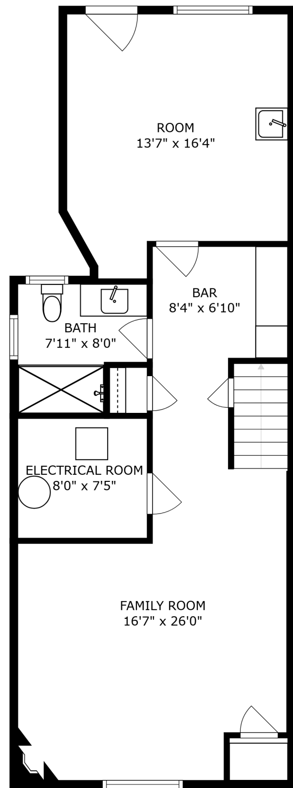
FLOOR 1
