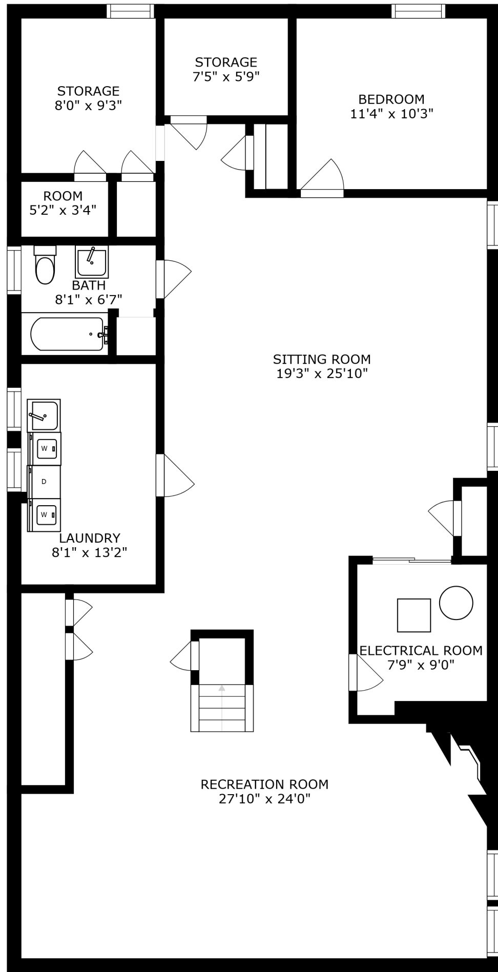
FLOOR 1
