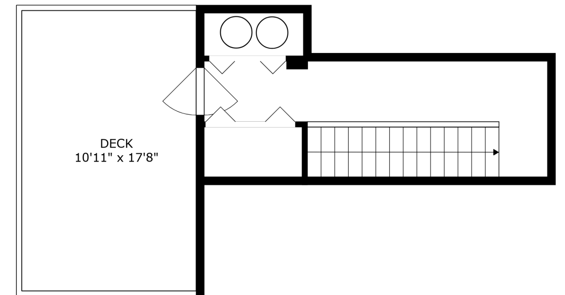
FLOOR 3
