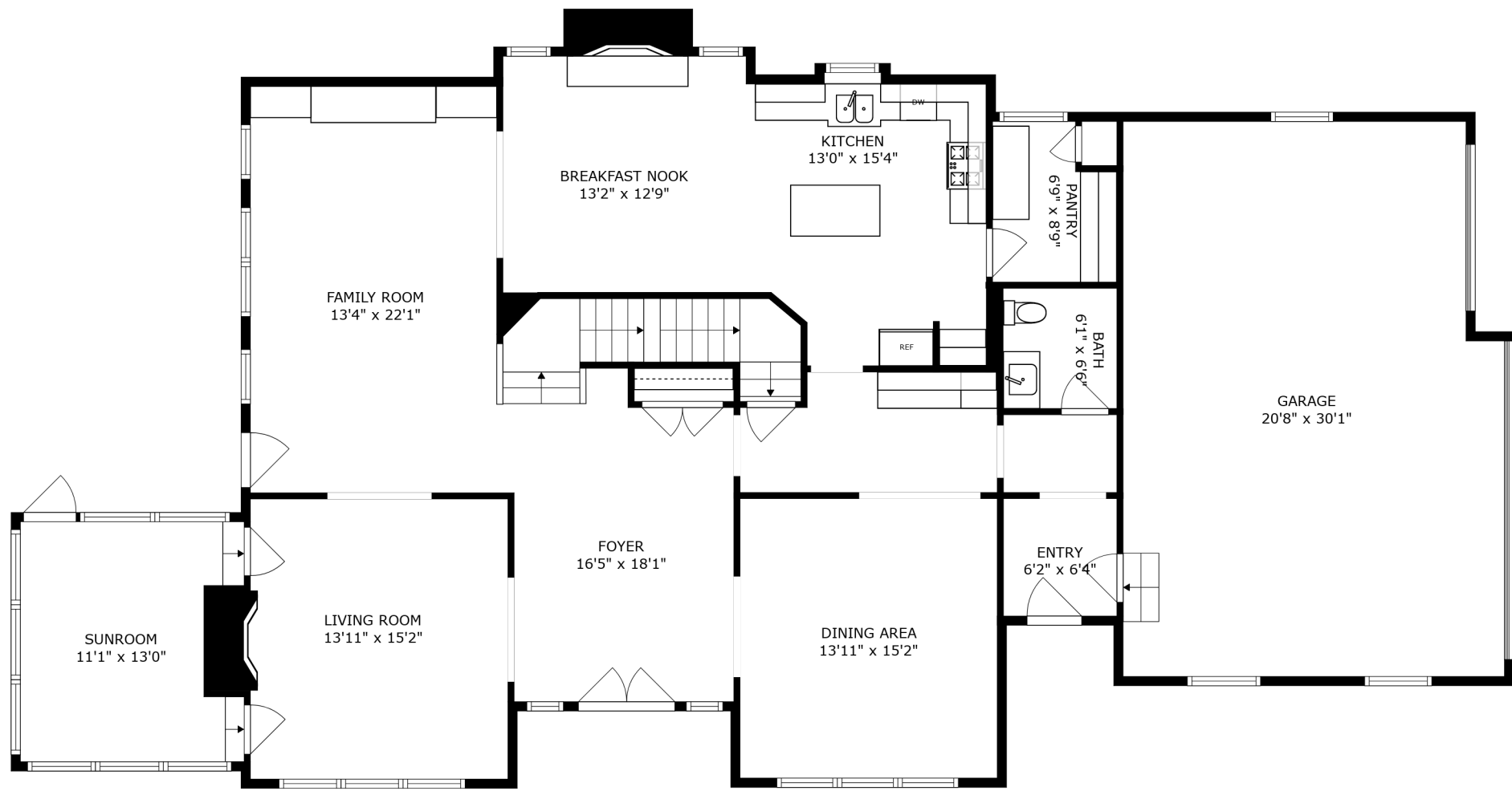
FLOOR 2
