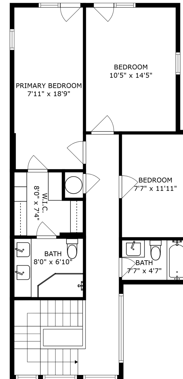
FLOOR 3
