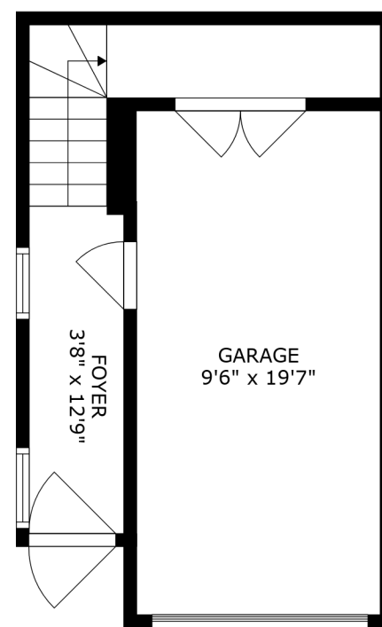
FLOOR 1
