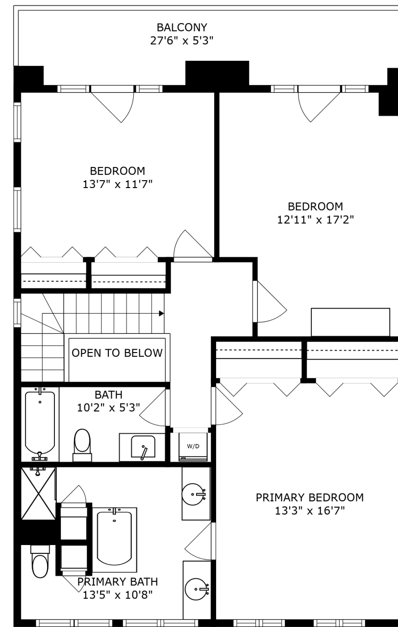
FLOOR 3
