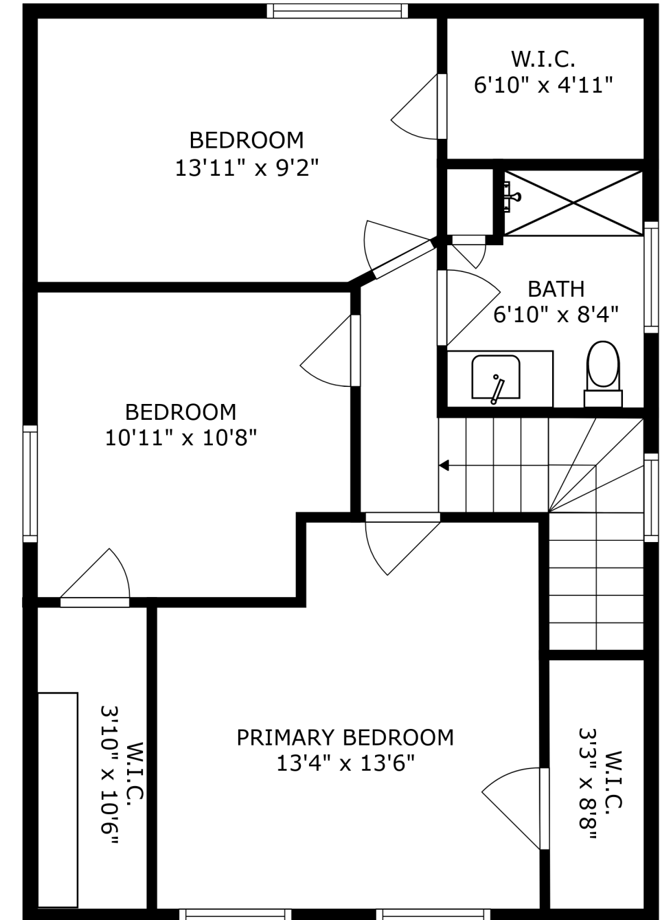
FLOOR 3
