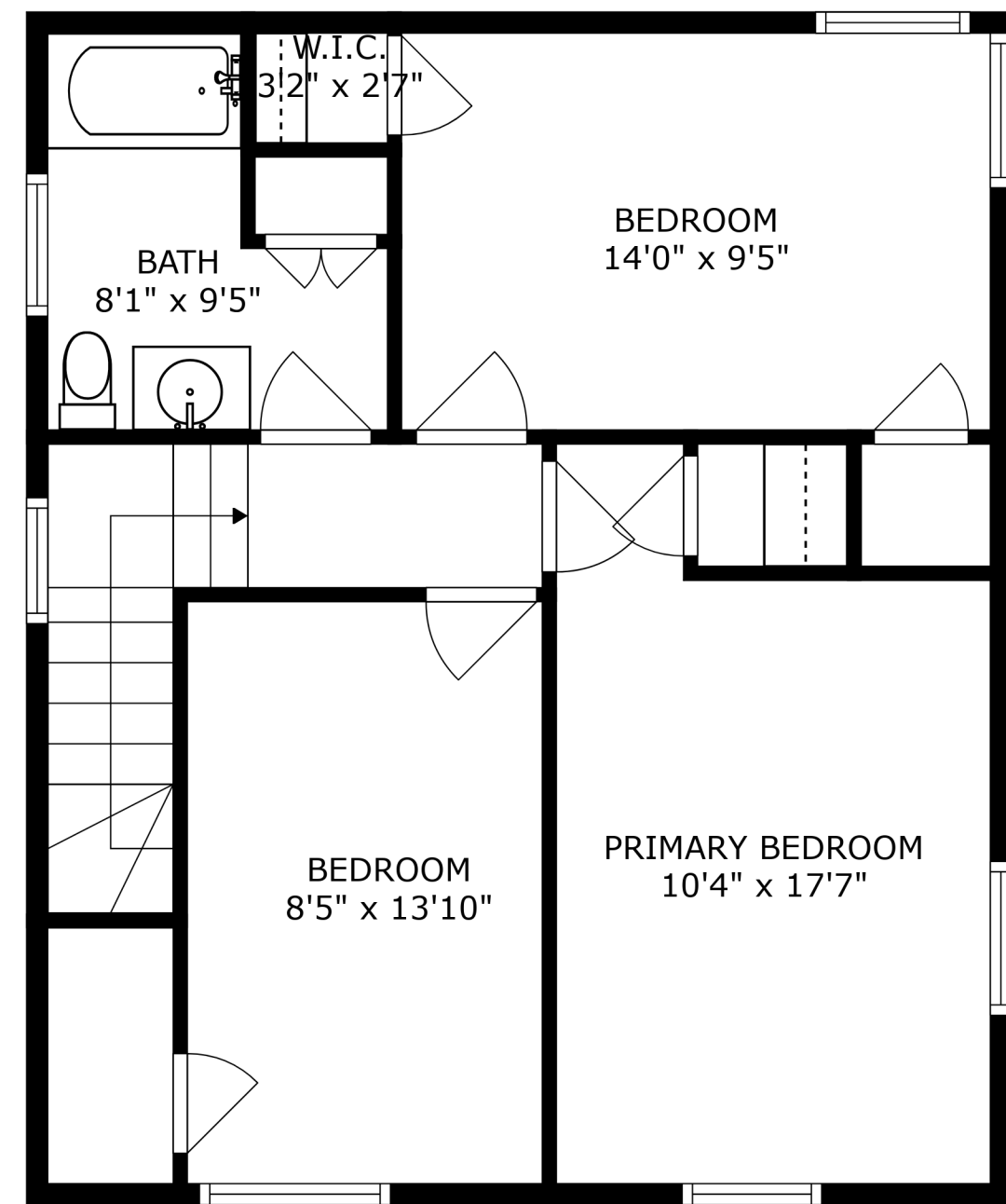
FLOOR 3
