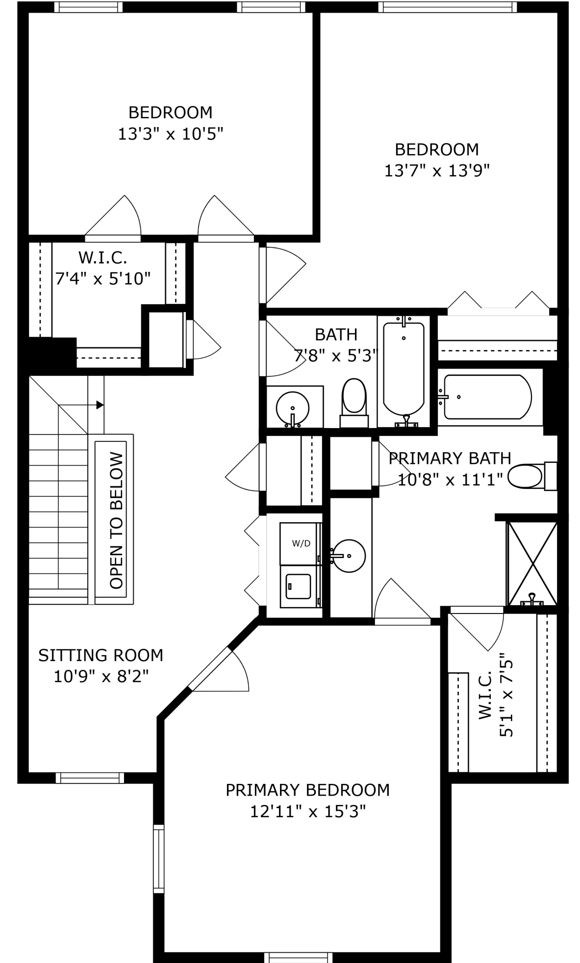
FLOOR 3
