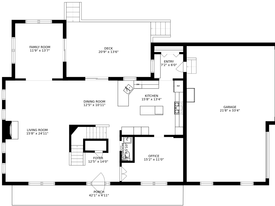
FLOOR 2
