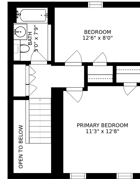
FLOOR 3
