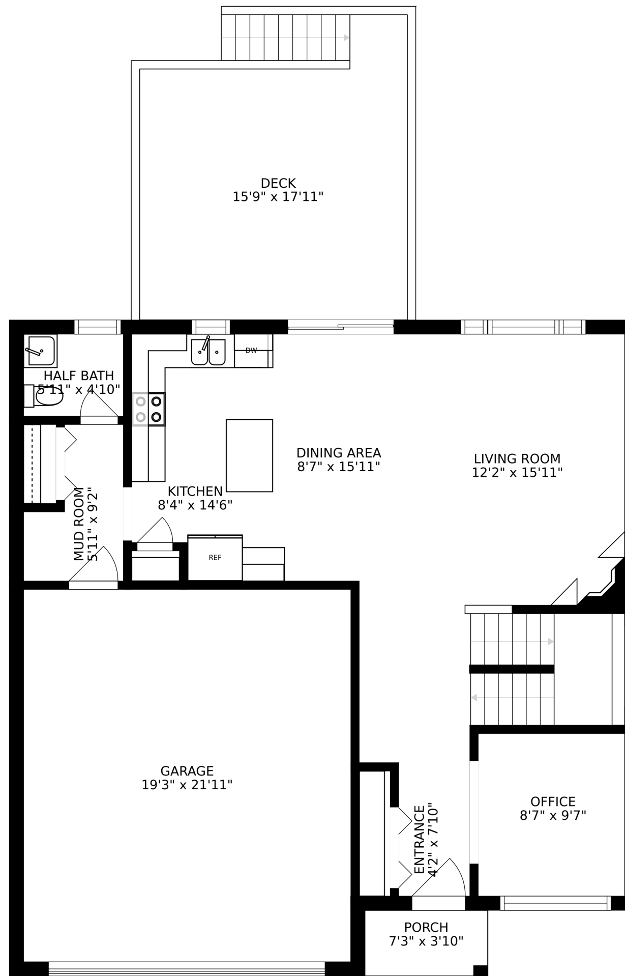
FLOOR 2
