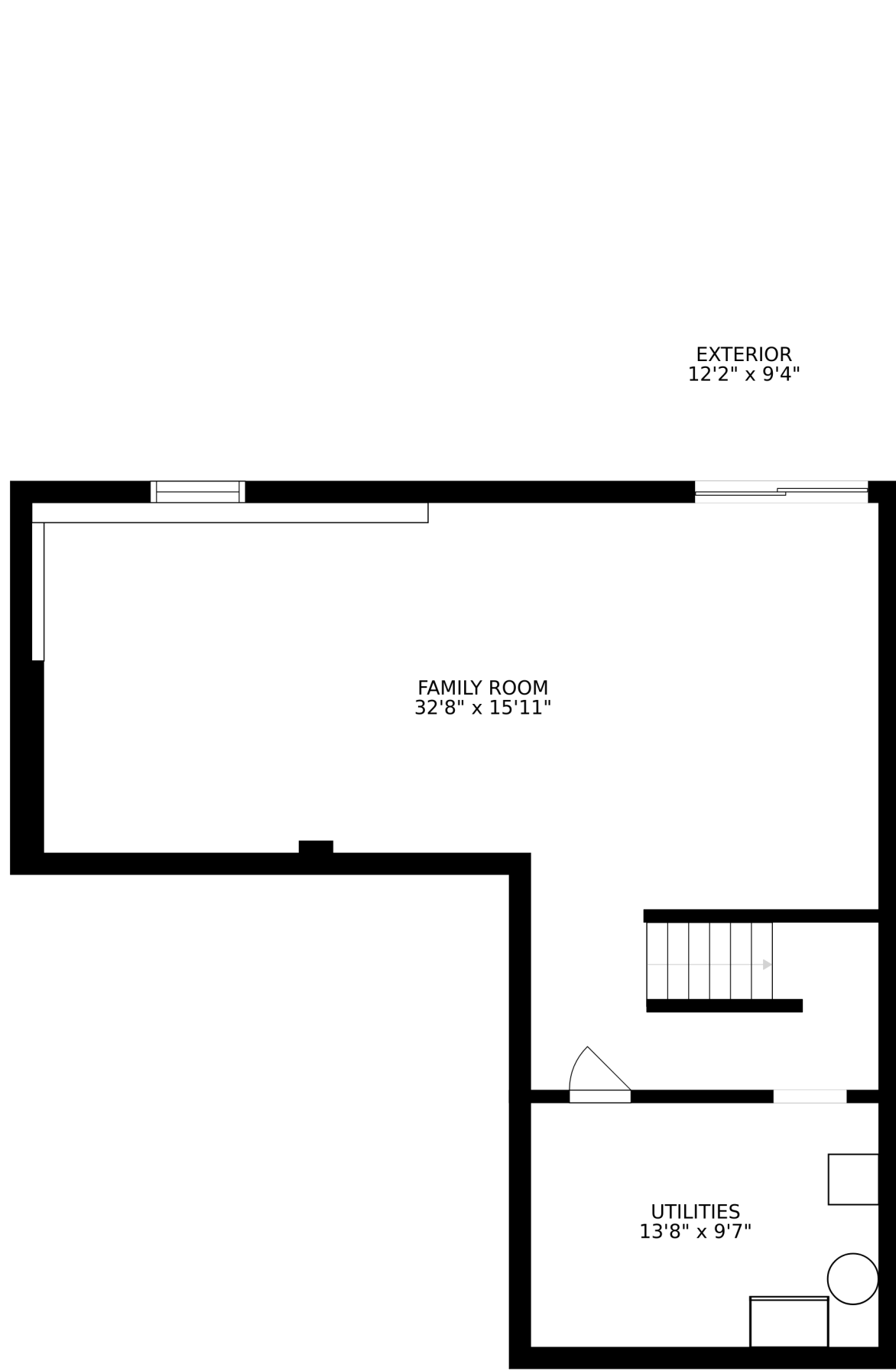
FLOOR 1
