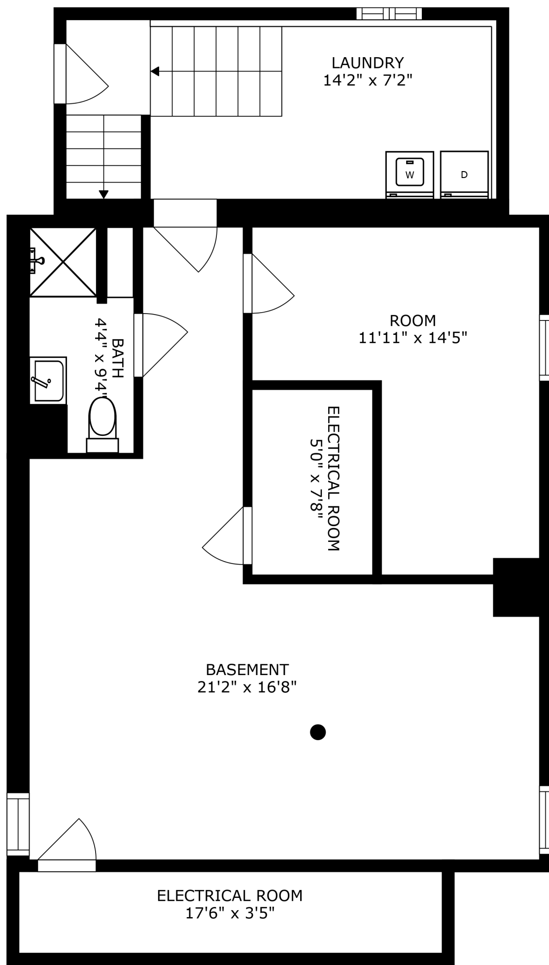
FLOOR 1
