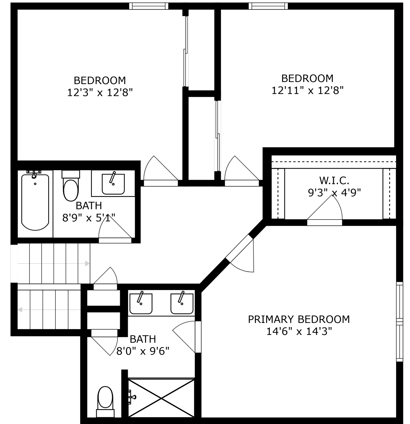
FLOOR 2
