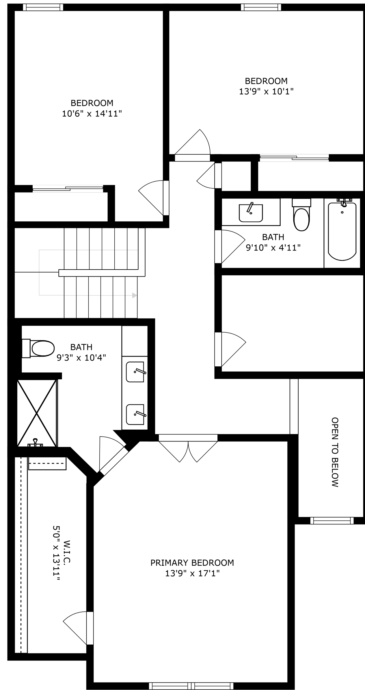
FLOOR 2
