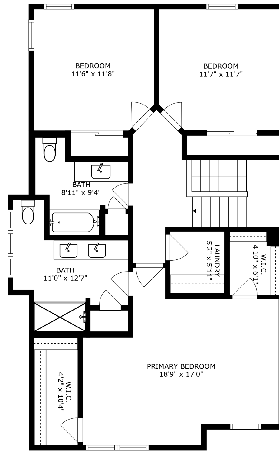
FLOOR 3
