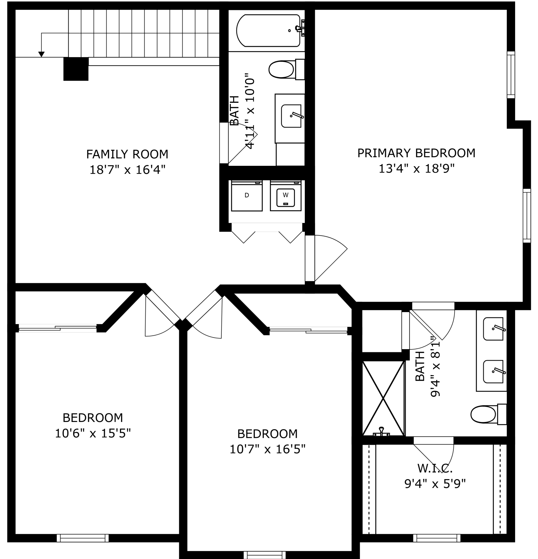
FLOOR 2
