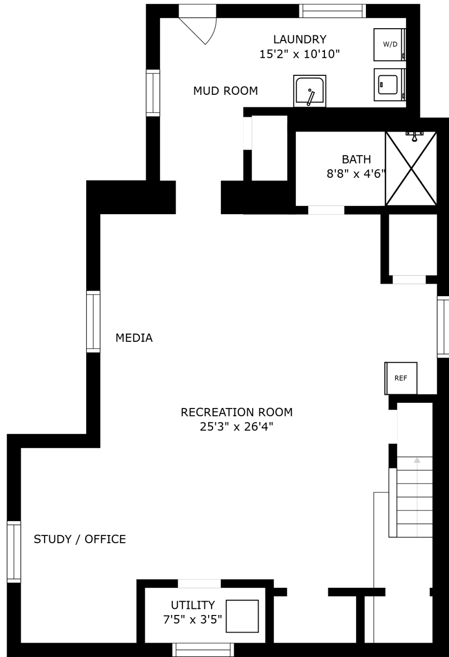
FLOOR 1
