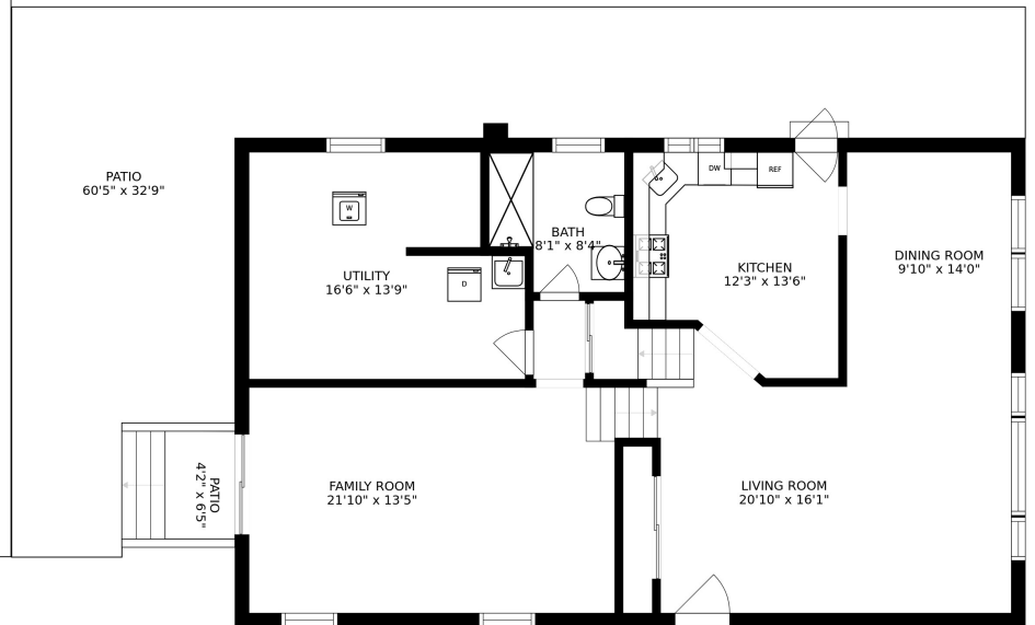
FLOOR 2
