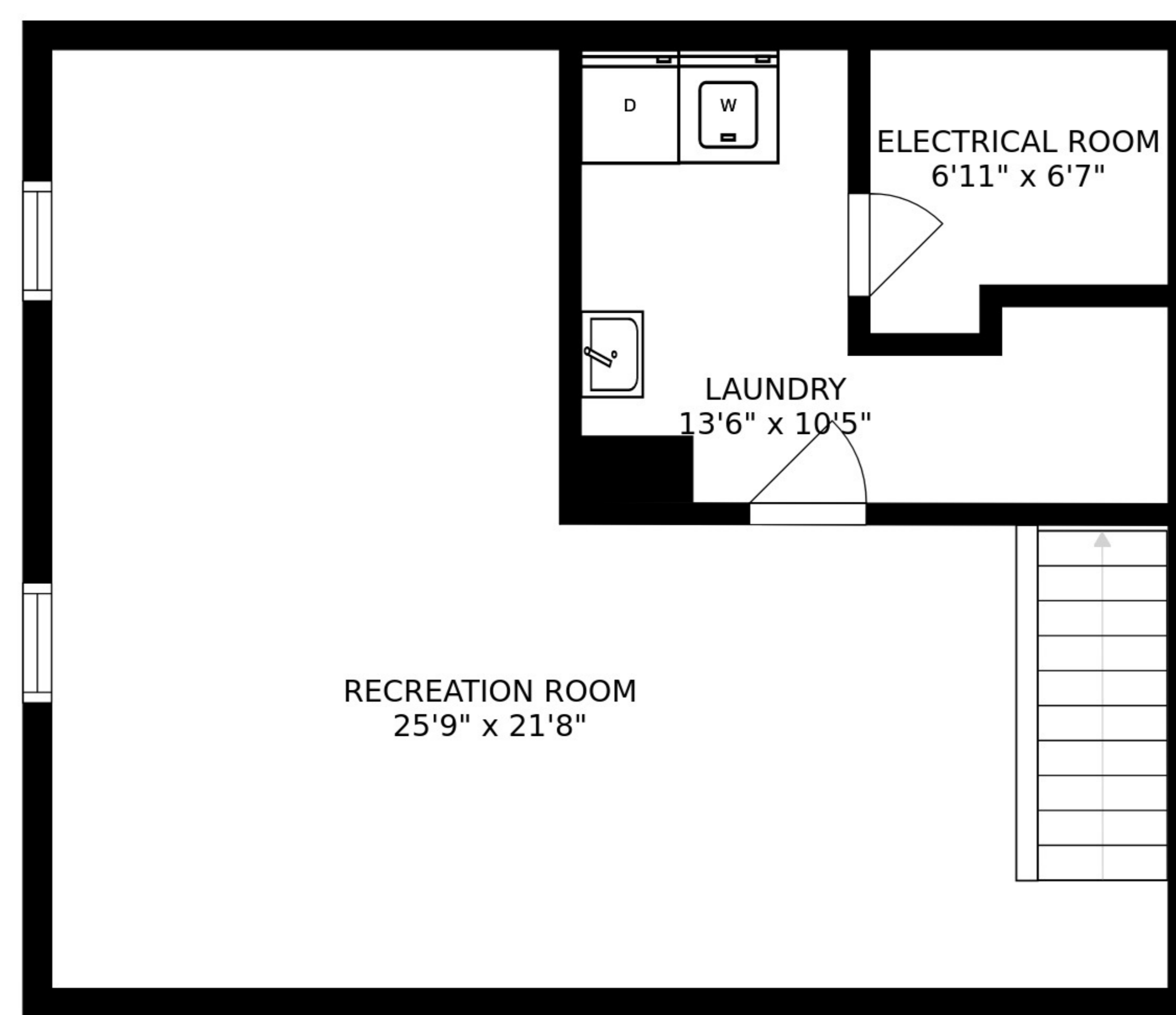
FLOOR 1
