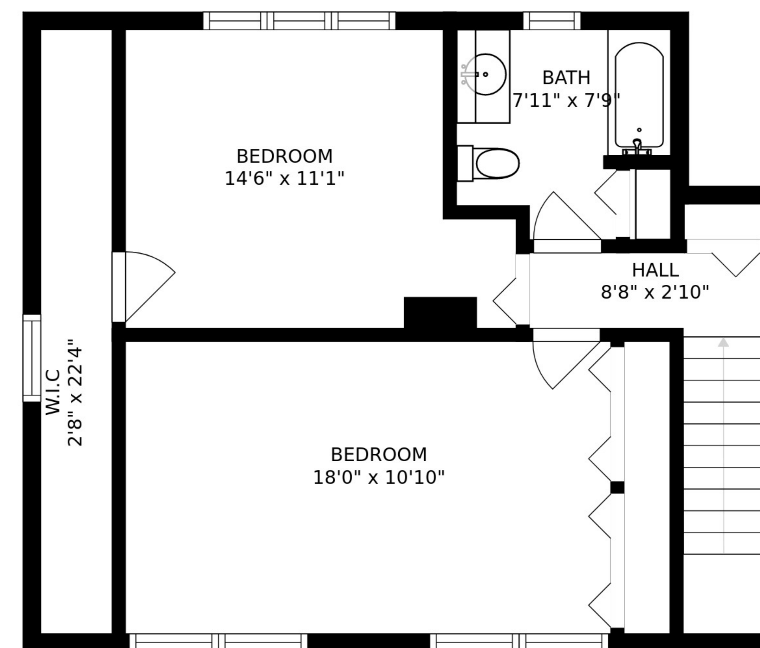
FLOOR 3
