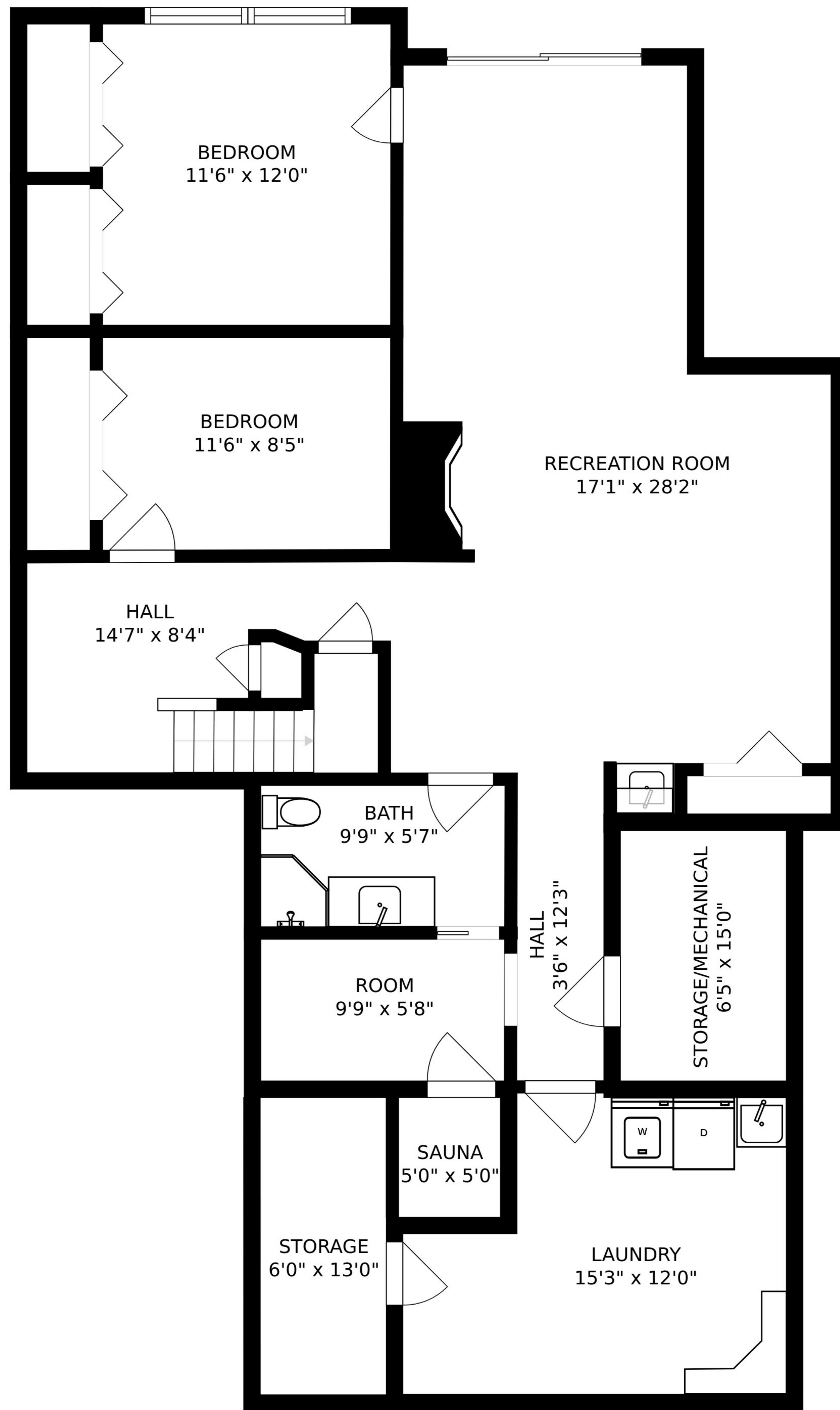
FLOOR 1
