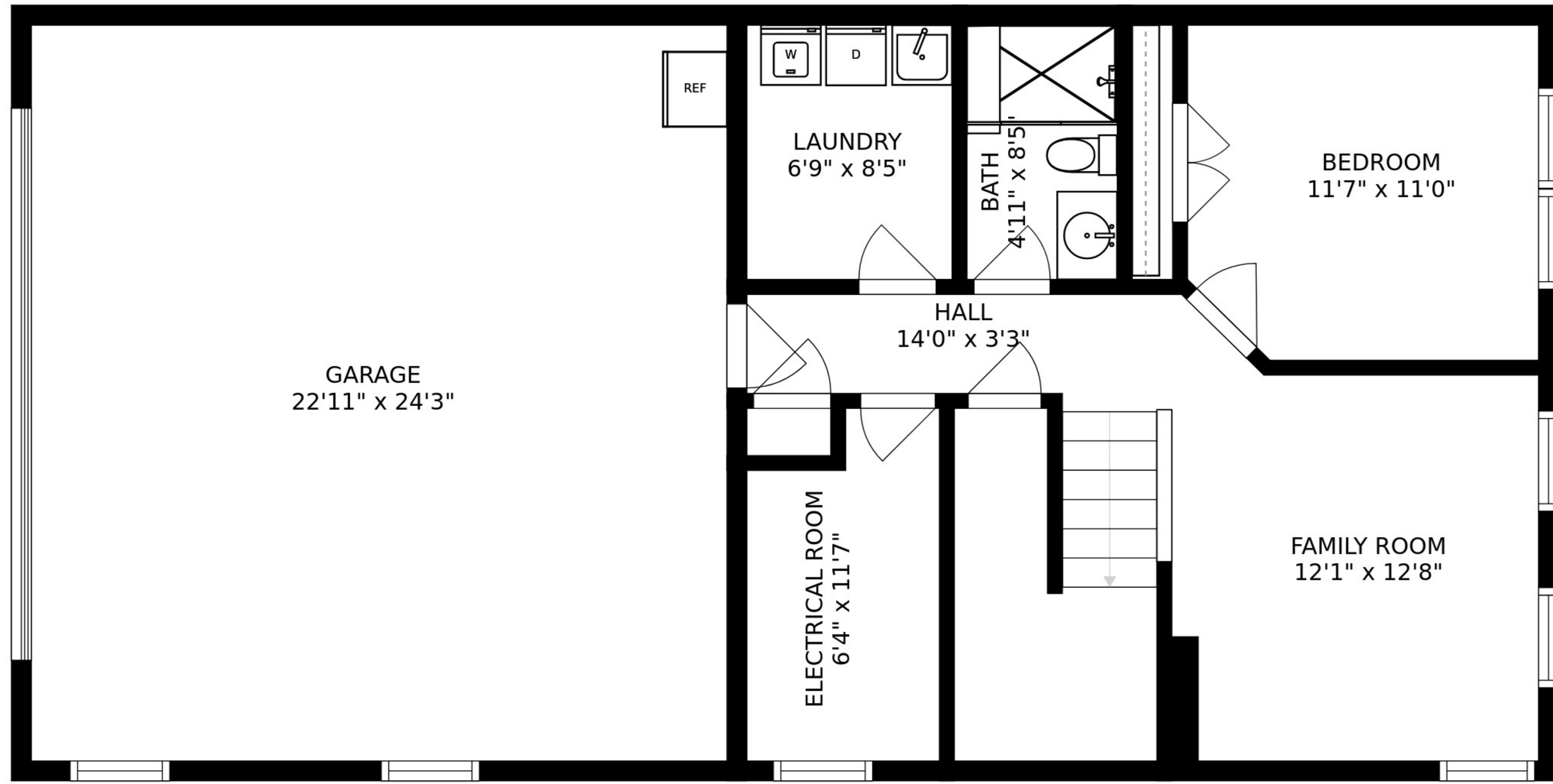
FLOOR 1
