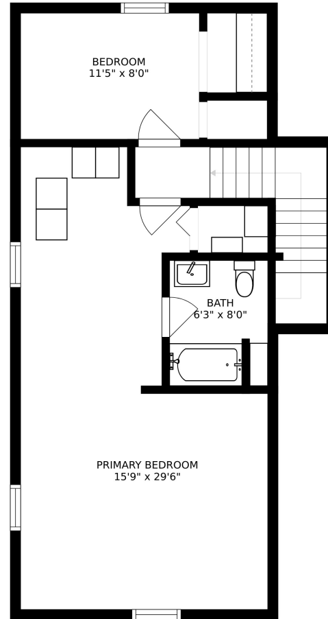
FLOOR 2
