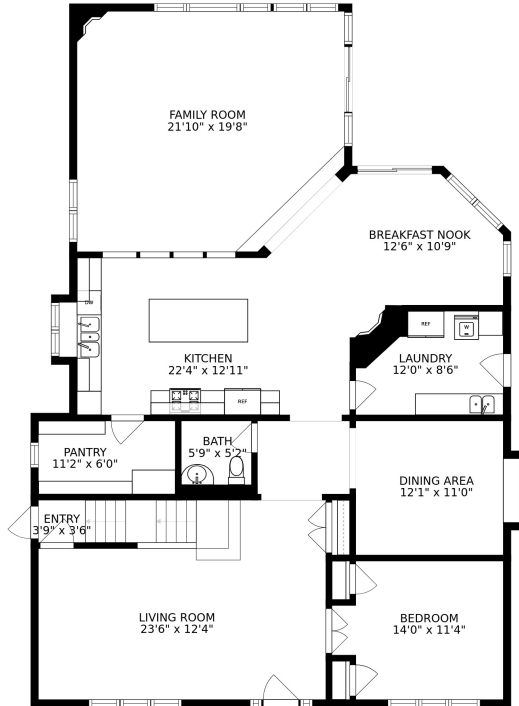
FLOOR 2
