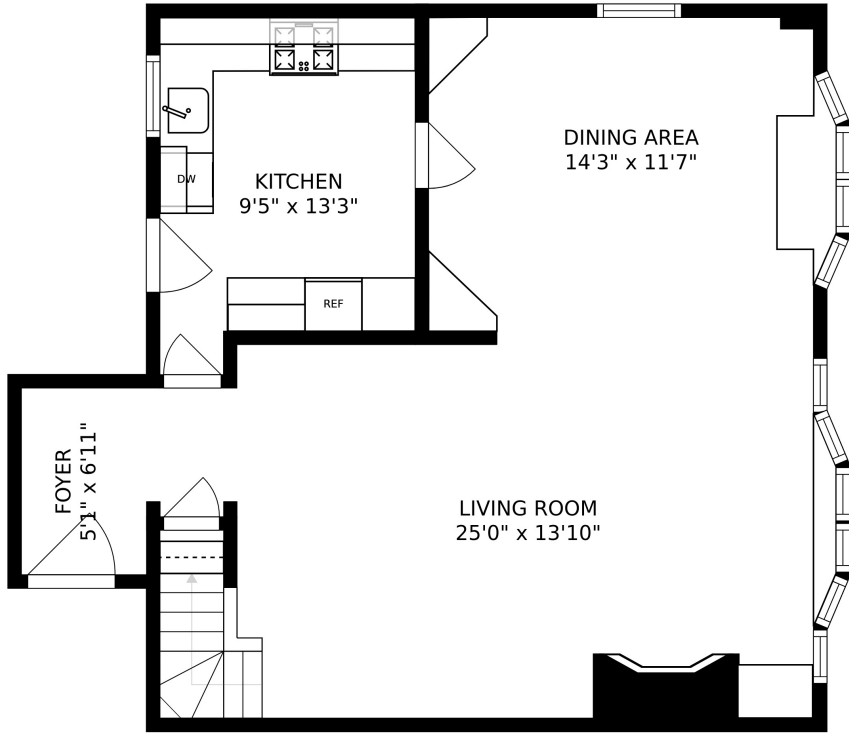
FLOOR 1
