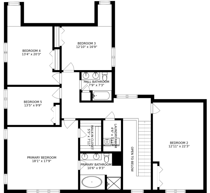
FLOOR 3
