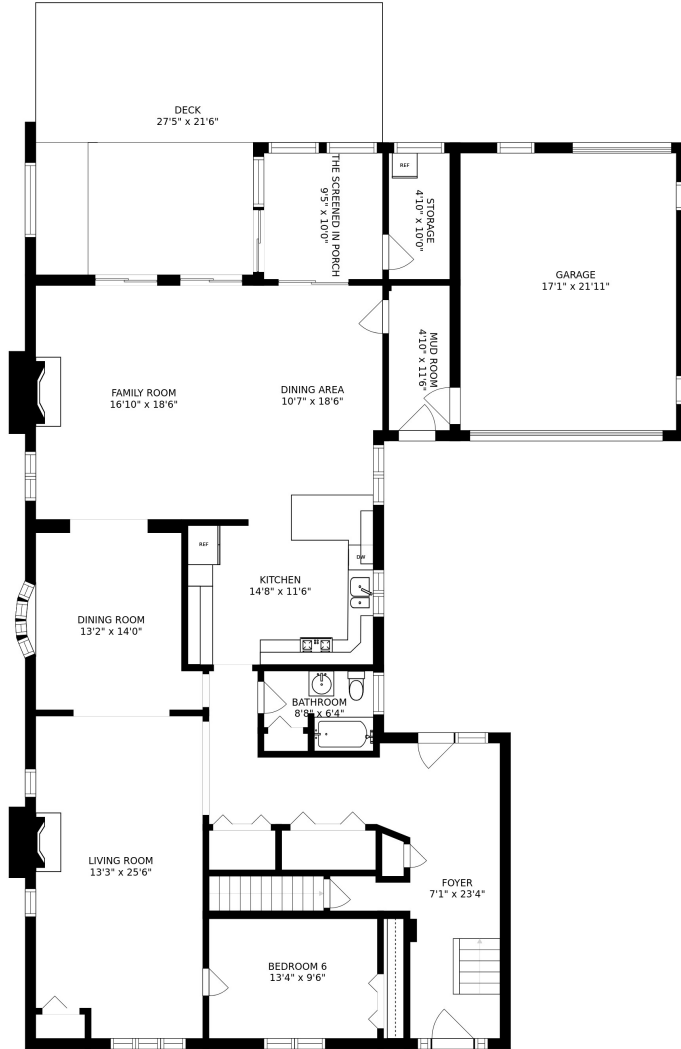
FLOOR 2
